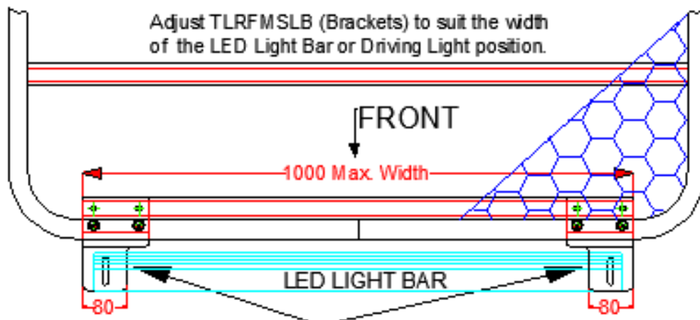
TLRFMSLB TLR FRONT MOUNT SPOTLIGHT - LIGHT BAR BRACKETS PLAN VIEW
